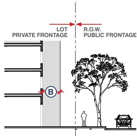
FIGURE 3.24: FORECOURT FRONTAGE SECTION
