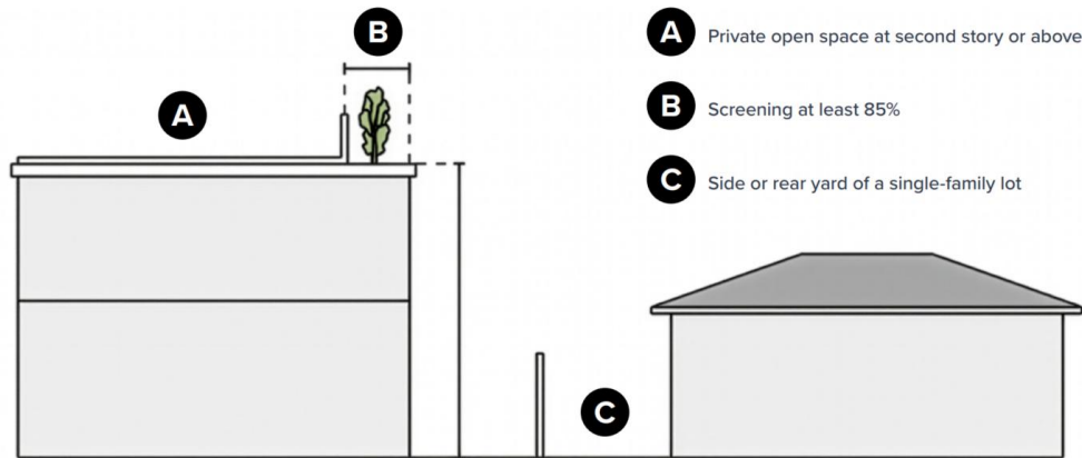
Figure 106-364-1. Private Open Space Screening Diagram
