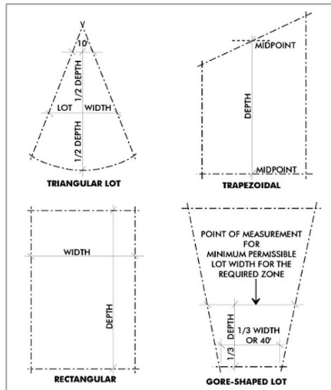
Figure 106-1179-3. Lot Width and Depth Measurements
