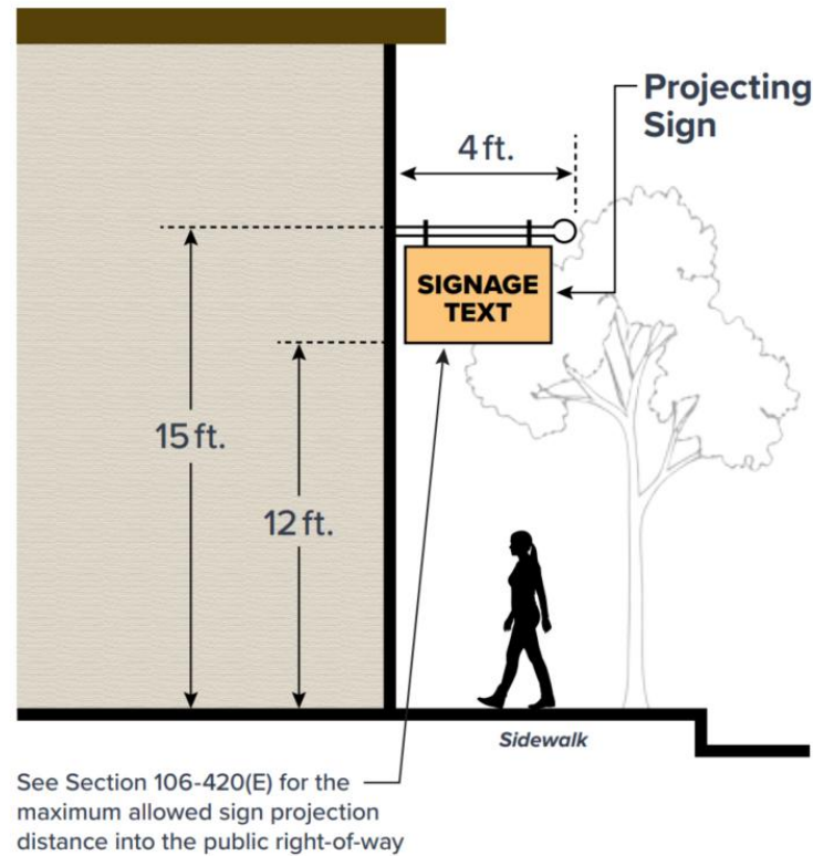
Figure 106-420-3. Projecting Signs
