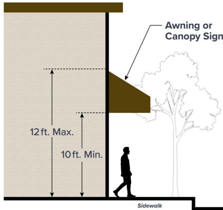
Figure 106-420-2. Awning and Canopy Sign
