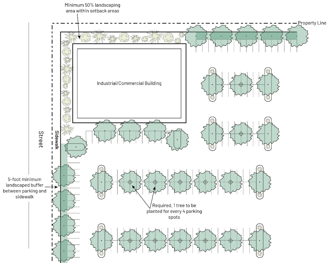
Figure 106-345-2. Commercial Parking Lot Landscaping Diagram
